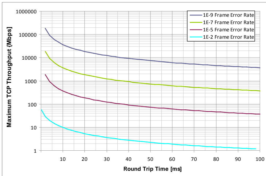
Figure 12. Frame Error/Loss Ratio Limits Maximum Throughput
